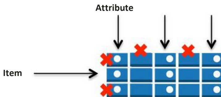
Figure 7: Database-level permissions
